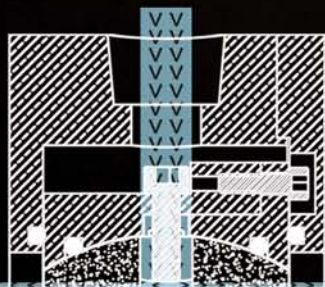
Inpro/Seal Smooth Bore Air Mizer cutaway with positive air purge Patent# 7,396,017
